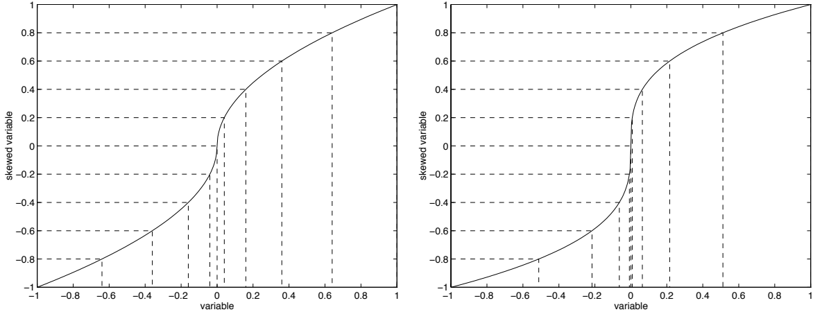
Figure 12: Skewing functions.
