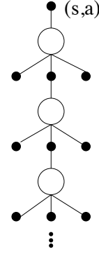
Figure 2. Backup diagram for the tree backup algorithm
