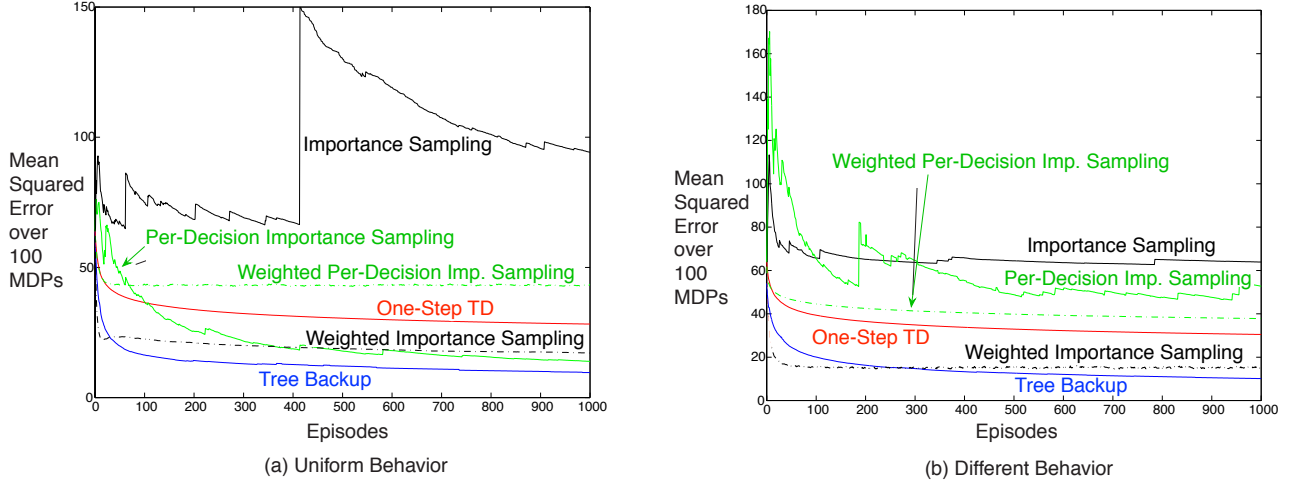
Figure 3. Average performance of all algorithms. On the left the behavior policy chose 50-50 from the two actions. On the right the behavior policy chose with 80-20 probabilities exactly opposite those of the target policy.
