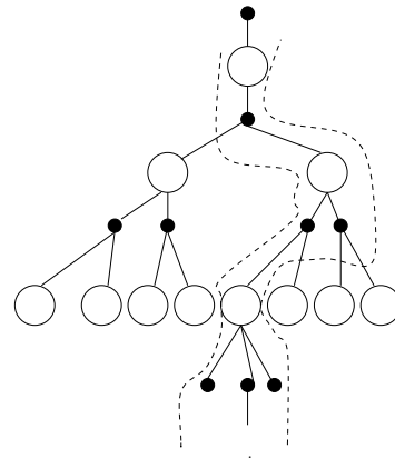
Figure 4. Full trajectory tree for an MDP
