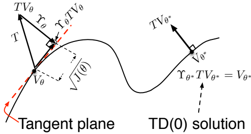
Figure 1: The MSPBE objective for nonlinear function approximation at two points in the value function space. The figure shows a point, V_\theta , at which, J(\theta) , is not 0 and a point, V_{\theta^*} , where J(\theta^*) = 0 , thus \Upsilon_{\theta^*} TV_{\theta^*} = V_{\theta^*} , so this is a TD(0) solution.
