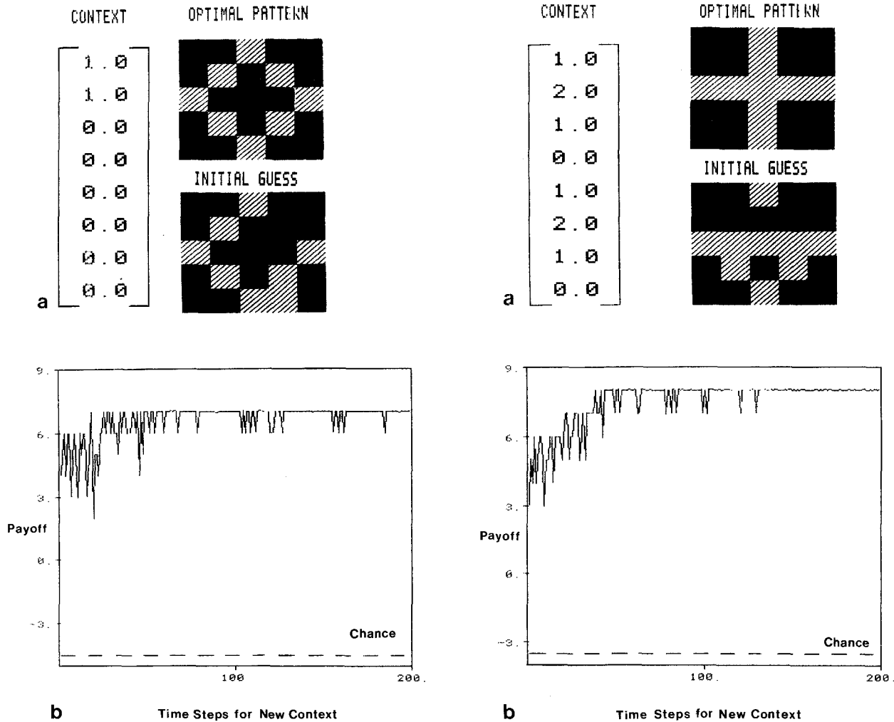
Fig. 9a and b. Example 4. With the associative matrix obtained after training in Example 2, a fragment of X^1 was presented as context. E implemented payoff function Z^1 . a The fragment of X^1 , the optimal pattern, and the initial guess. b ASN payoff as the search continues
