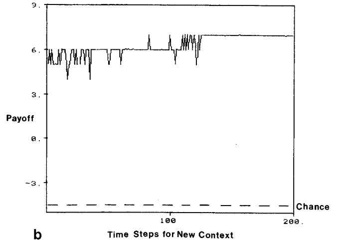
Fig. 8a and b. Example 3. With the associative matrix obtained after training in Example 2, context vector X^1 of Fig. 7a was corrupted by additive noise and presented to the ASN. a The corrupted context vector, the optimal output pattern, and the ASN’s initial guess b ASN payoff as it searches for the optimal output pattern
