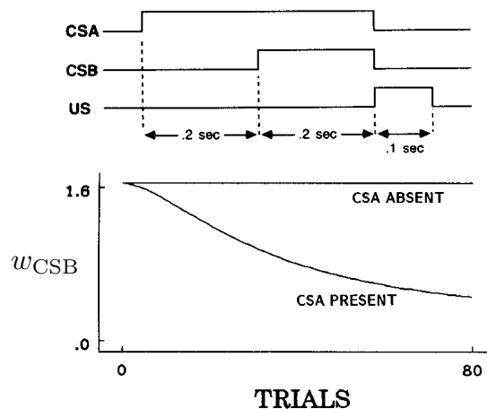
Figure 14.4: Temporal primacy overriding blocking in the TD model. Adapted from Sutton and Barto (1990).
