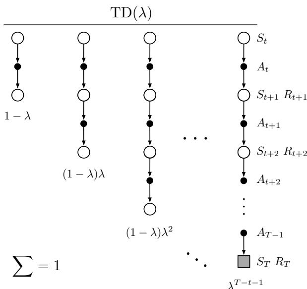
Figure 12.1: The backup diagram for \text{TD}(\lambda) . If \lambda = 0 , then the overall update reduces to its first component, the one-step TD update, whereas if \lambda = 1 , then the overall update reduces to its last component, the Monte Carlo update.
